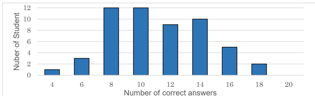
Figure 1. Score distribution of CT Test 2024.
